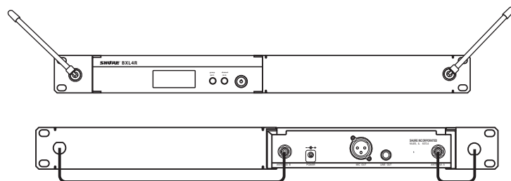
Antenna Connection Diagram
